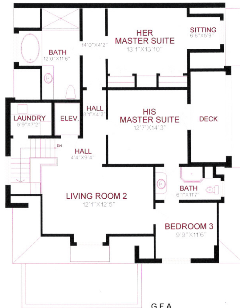
THIRD FLOOR
