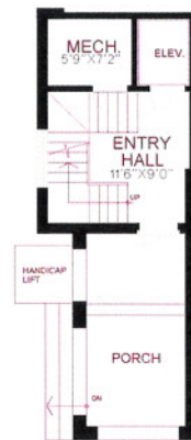
FIRST FLOOR
